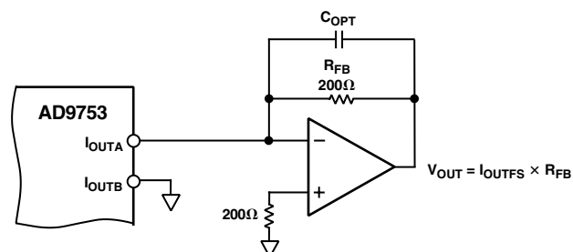
Figure 24. Unipolar Buffered Voltage Output
