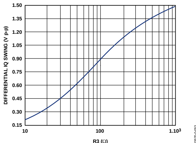
Figure 52. Relationship Between R3 in Figure 51 and Peak Baseband Input Voltage
