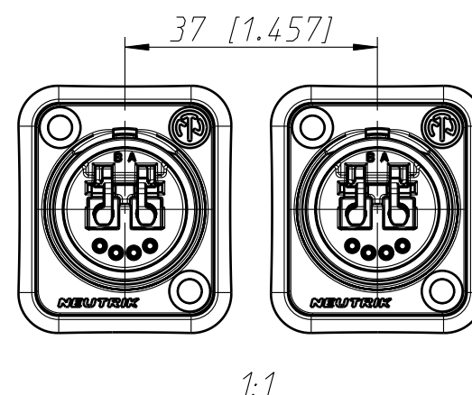
Einbauabstand assembling distance
