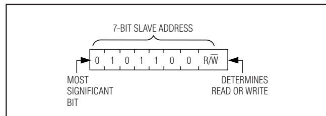
Figure 4. Slave Address and the R/\bar{W} Bit
