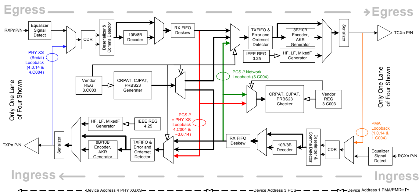
FIGURE 6. BLOCK DIAGRAM OF BIST OPERATION
