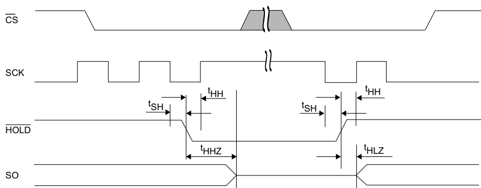
Figure 26. \overline{HOLD} Timing
