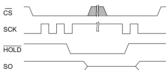
Figure 23. \overline{HOLD} Operation
