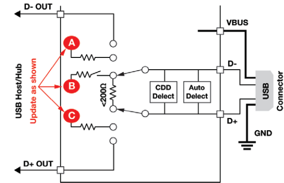
USB charging controller handshake interface.
