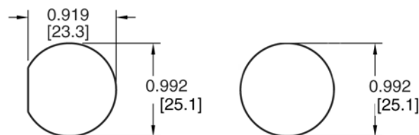
RECOMMENDED PANEL CUT-OUT ±0.003 [±0.1]
