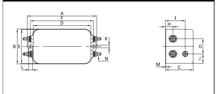
Connection style -08, 20 A types
