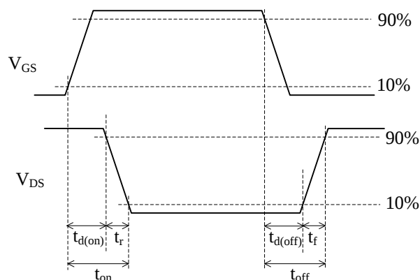
(b) Waveform
