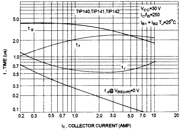
SWITCHING TIME
