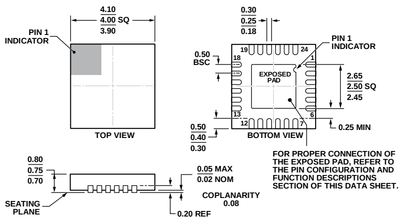
Figure 79. 24-Lead Lead Frame Chip Scale Package [LFCSP_WQ] 4 mm x 4 mm Body, Very Very Thin Quad (CP-24-7) Dimensions shown in millimeters
