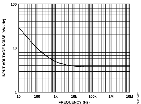
Figure 44. Voltage Noise Spectral Density, Referred to Input
