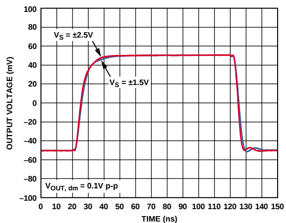
Figure 56. V_{OCM} Small Signal Transient Response
