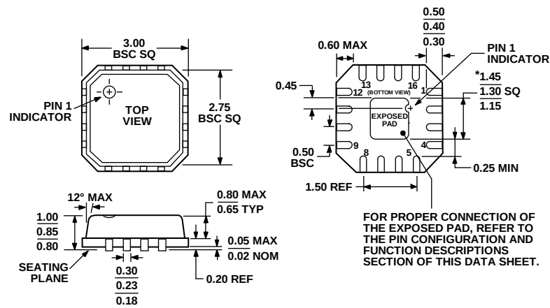
Figure 77. 16-Lead Lead Frame Chip Scale Package [LFCSP_VQ] 3 mm x 3 mm Body, Very Thin Quad (CP-16-2) Dimensions shown in millimeters
