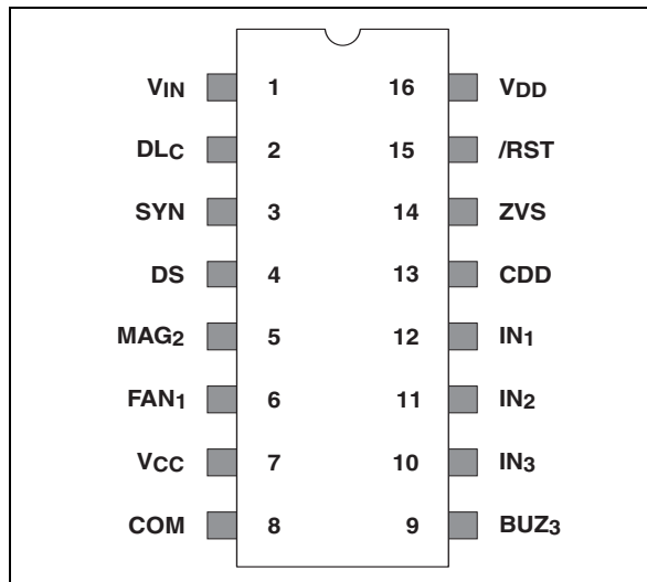
Figure 2: Pin-out connections
