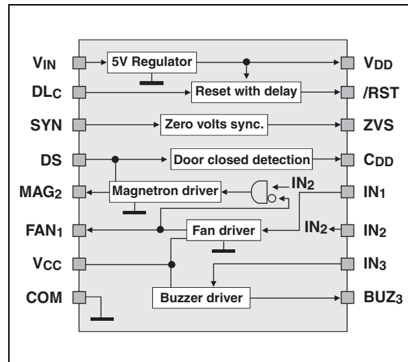
Figure 3: Block diagram
