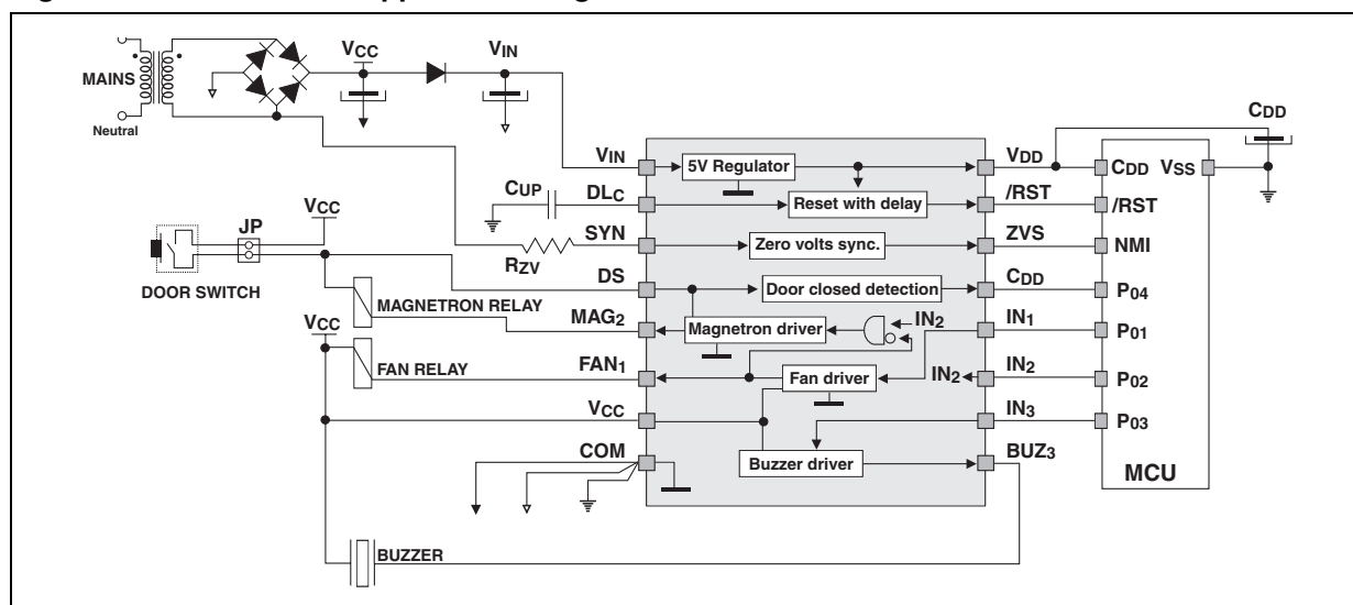
Figure 1: STCC02 Based Application Diagram
