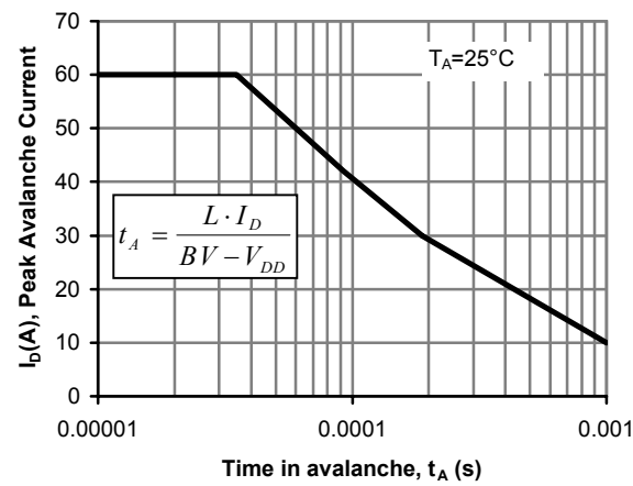
Figure 12: Avalanche capability
