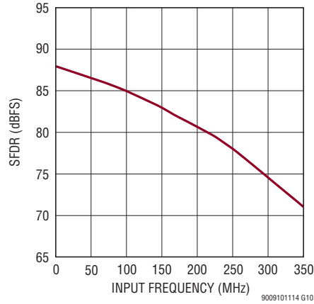
LTM9011-14: SFDR vs Input Frequency, -1dBFS, 2V Range, 125Msps
