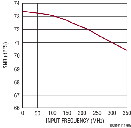
LTM9011-14: SNR vs Input Frequency, -1dBFS, 2V Range, 125Msps
