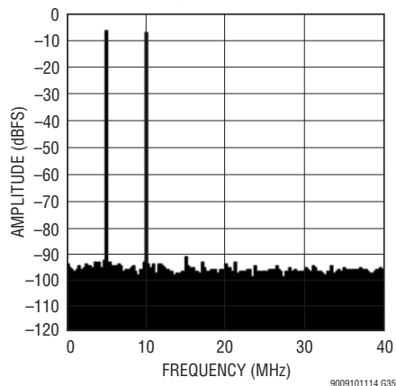
LTM9009-14: 8k Point 2-Tone FFT, f_{IN} = 70\text{MHz} , 75\text{MHz} , -7\text{dBFS} per Tone, 80Mps
