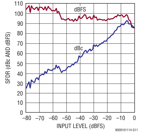
LTM9011-14: SFDR vs Input Level, f_{IN} = 70\text{MHz} , 2V Range, 125Msps
