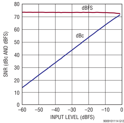
LTM9011-14: SNR vs Input Level, f_{IN} = 70\text{MHz} , 2V Range, 125Msps
