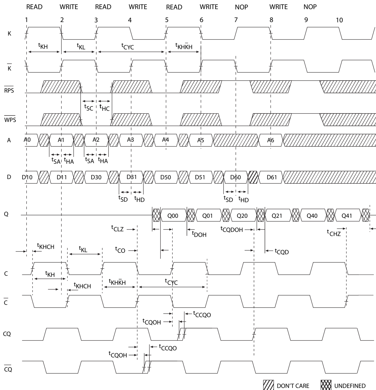
Figure 6. Read/Write/Deselect Sequence [26, 27, 28]
