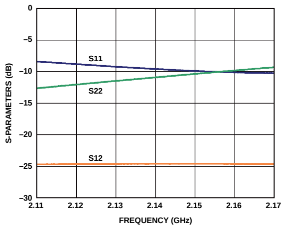
Figure 18. Input Return Loss (S11), Output Return Loss (S22), and Reverse Isolation (S12) vs. Frequency
