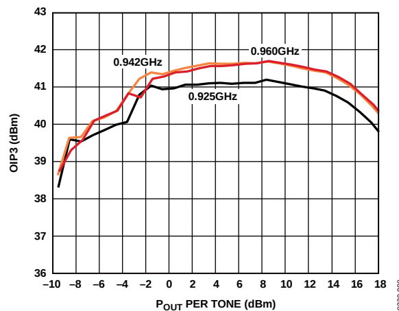
Figure 8. OIP3 vs. P_{OUT} and Frequency
