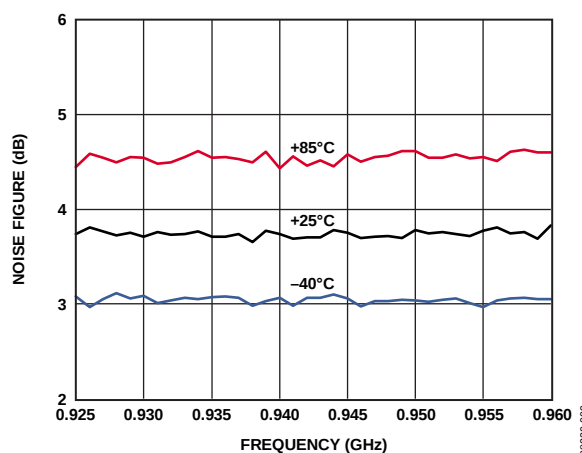
Figure 9. Noise Figure vs. Frequency and Temperature
