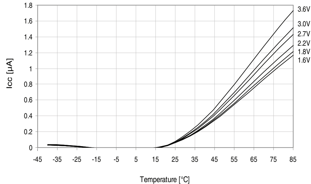
Figure 33-255. Power-down mode supply current vs. temperature. All functions disabled.
