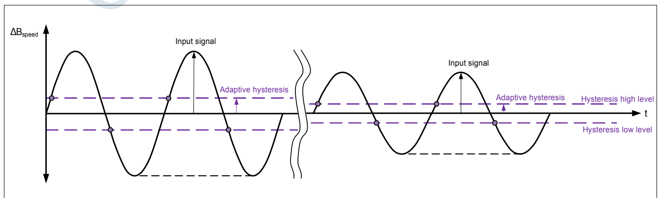
Figure 5 Adaptive Hysteresis
