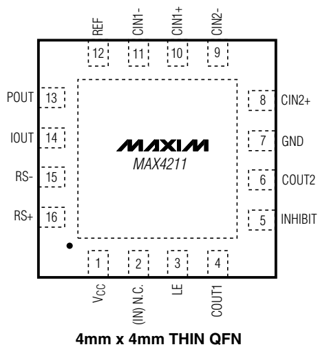
4mm x 4mm THIN QFN
