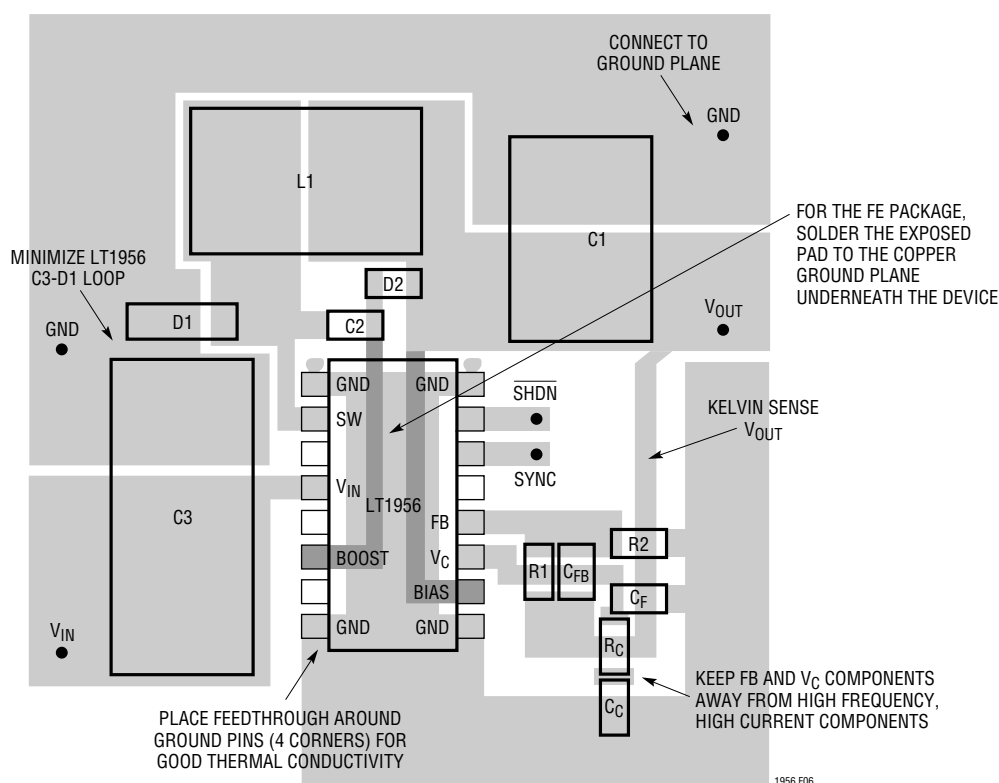
Figure 6. Suggested Layout
