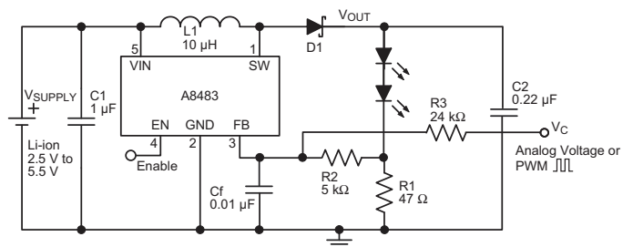
Figure 8. WLED Backlighting. (Circuit also shown in figure 5.)
