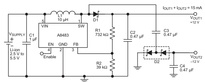
Figure 2. Small LCD Bias Supply. Li+ battery to \pm 12 V.
