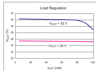
Figure 19. Load Regulation for LCD TV, Plasma TV Bias, FED Display, Varactor Diode Bias; V_{SUPPLY} = 12 \text{ V} (circuit also shown in figure 4). The A8483 can operate with a V_{SUPPLY} from 0.9 to 18 V with a separate bias supply to operate the A8483 in the normal V_{IN} range. The bias voltage can be supplied by an external power supply, such as 3.3 or 5 V, or by using a suitable Zener diode, V_Z , for V_{SUPPLY} > 10 \text{ V} .
