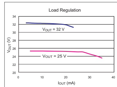
Figure 18. Load Regulation for LCD TV, Plasma TV Bias, FED Display, Varactor Diode Bias; V_{SUPPLY} = 5 \text{ V} (circuit also shown in figure 3)
