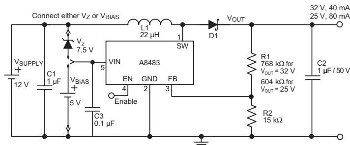
Figure 19. Load Regulation for LCD TV, Plasma TV Bias, FED Display, Varactor Diode Bias; V_{SUPPLY} = 12 \text{ V} (circuit also shown in figure 4). The A8483 can operate with a V_{SUPPLY} from 0.9 to 18 V with a separate bias supply to operate the A8483 in the normal V_{IN} range. The bias voltage can be supplied by an external power supply, such as 3.3 or 5 V, or by using a suitable Zener diode, V_Z , for V_{SUPPLY} > 10 \text{ V} .
