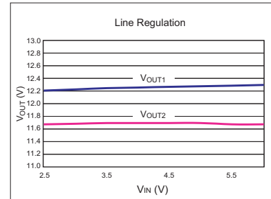
Figure 17. Line Regulation Performance for Small LCD Bias Supply, I_{OUT1} = I_{OUT2} = 7.5 \text{ mA} (circuit also shown in figure 2)
