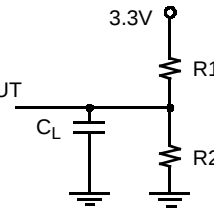
(a) LVTTTL AC Test Load
