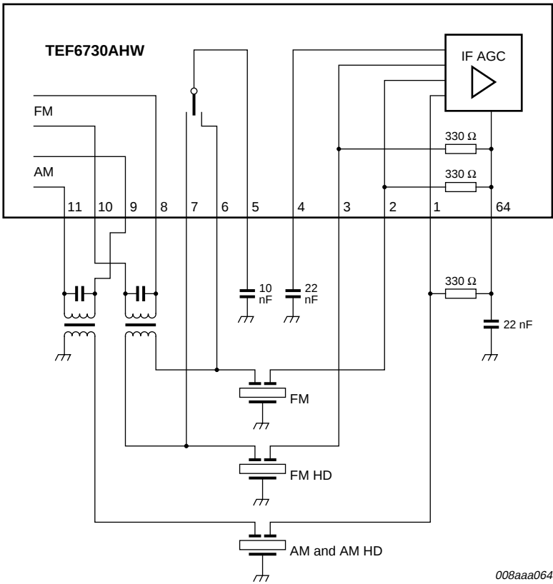
Fig 30. FM, AM, AM HD and FM HD mode
