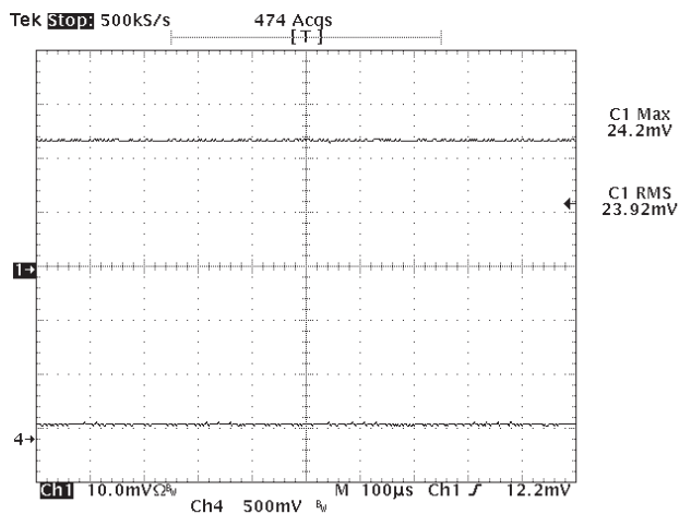
Figure 11: Short Circuit Characteristic (Channel 1: Output Current at 10A/div, Channel 4: Output Voltage)
