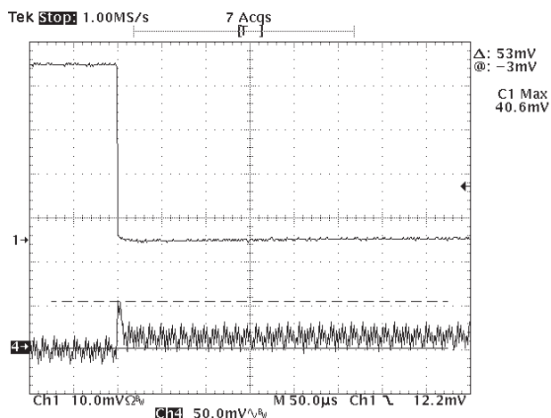
Figure 13: Transient Response 75 - 50% (Channel 1: Current load step at 2A/div, Channel 4: Output Voltage deviation)
