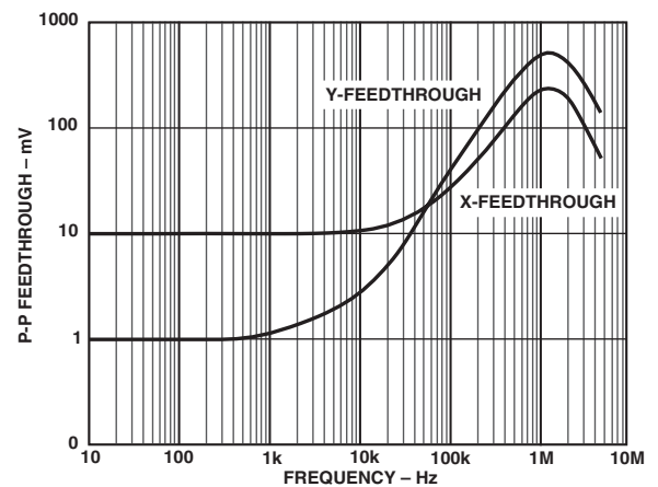
TPC 6. AC Feedthrough vs. Frequency
