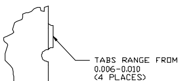
PHYSICAL DIMENSIONS
