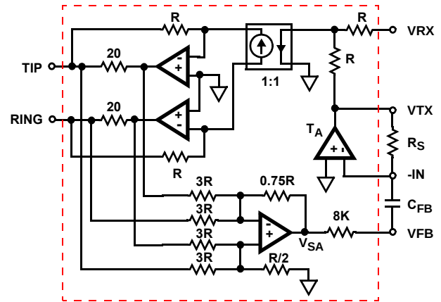
FIGURE 6. AC SIGNAL TRANSMISSION MODEL
