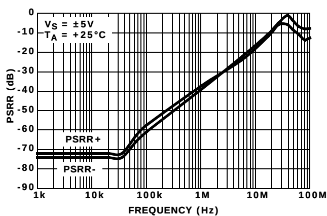
FIGURE 22. PSRR vs FREQUENCY
