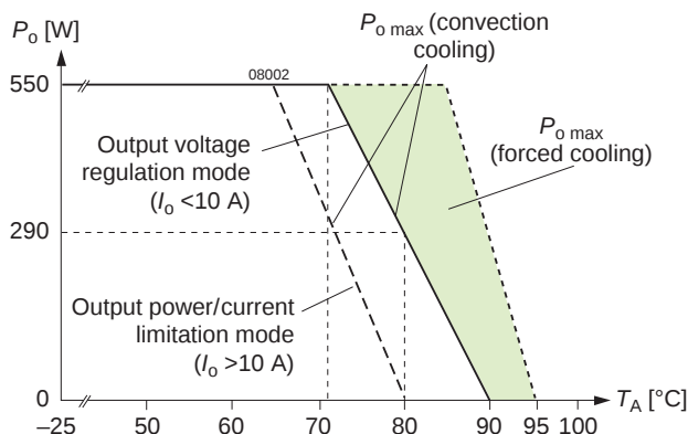
Fig. 42 Output power versus ambient temperature of T17xx
