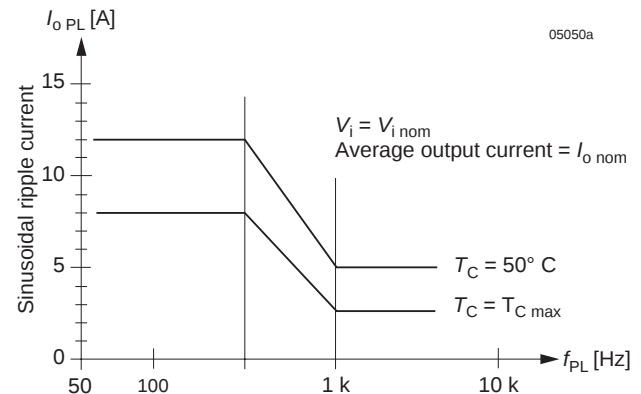
Fig. 10 Maximum AC ripple output current superimposed on the average output current I_{O\text{ nom}} for LT1701.
