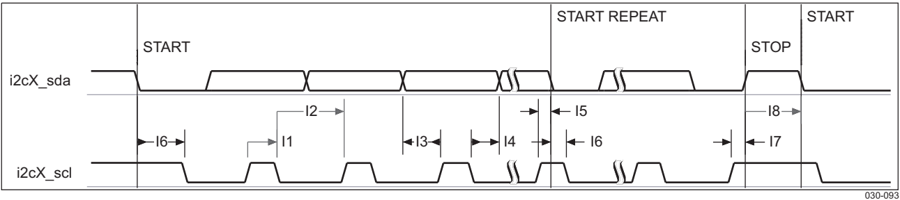
Figure 6-53. I 2 C – Standard/Fast Mode
