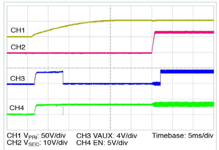
Figure 17 — Start up from application of V_{PRI\_DC} = 54V, 20% I_{OUT} , 100% C_{SEC\_OUT\_EXT}
