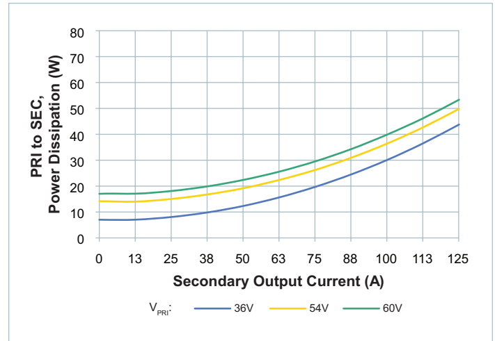
Figure 11 — Power dissipation at T_{CASE} = 80^{\circ}\text{C}
