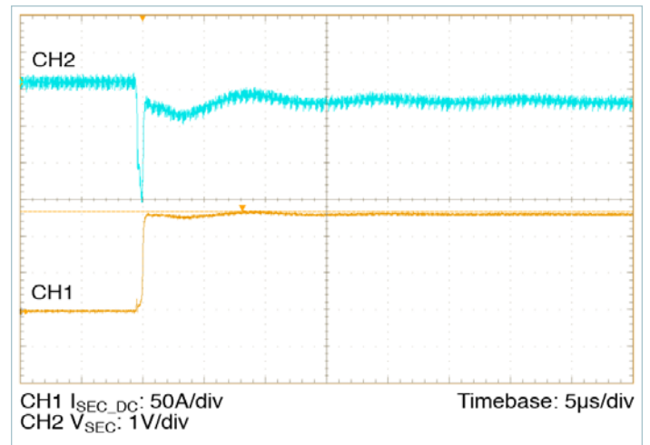
Figure 15 — 0A – 130A transient response: C_{PRI\_IN\_EXT} = 2700 \mu F, no external C_{SEC\_OUT\_EXT}
