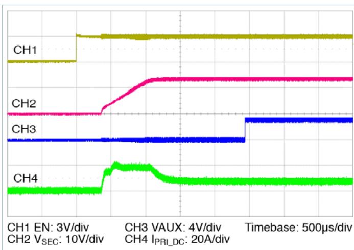
Figure 18 — Start up from application of EN with pre-applied V_{PRI\_DC} = 54V, 20% I_{SEC\_DC} , 100% C_{SEC\_OUT\_EXT}
