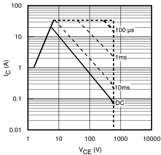
Fig. 3 - Forward SOA T_C = 25^\circ C ; T_J \leq 150^\circ C
