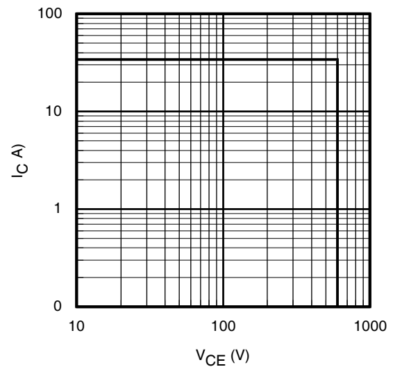
Fig. 4 - Reverse Bias SOA T_J = 150^\circ C ; V_{GE} = 15V
