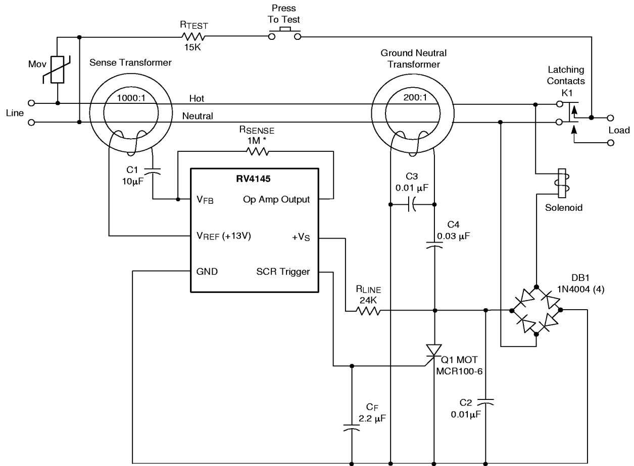
Figure 1. GFI Application Circuit (Three-Wire Outlet)
