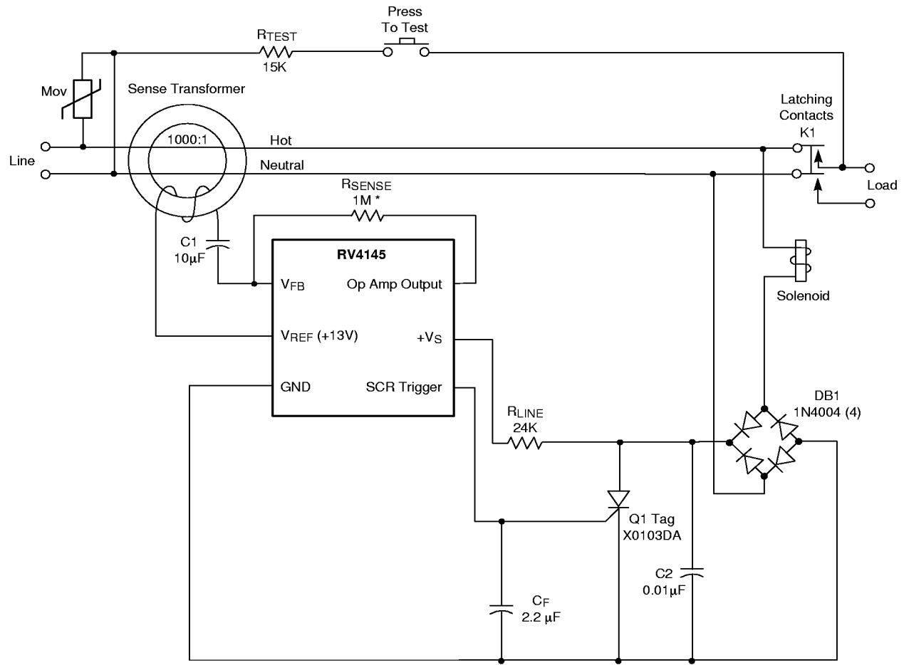
Figure 2. GFI Application Circuit (Two-Wire Outlet)
