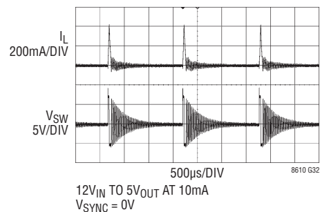
Switching Waveforms
