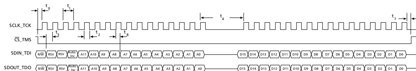
Figure 4-27: Write Mode
