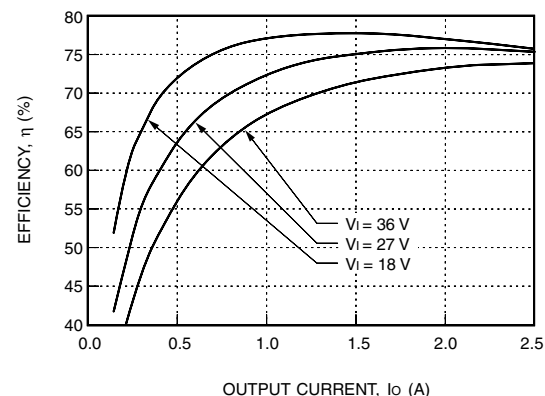
Figure 20. LC010F Typical Efficiency vs. Output Current at T_c = 25\text{ }^{\circ}\text{C}
