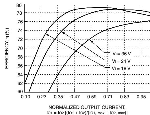
Figure 21. LC010AJ, BK, CL Typical Efficiency vs. Normalized Output Current at T_c = 25\text{ }^{\circ}\text{C}
