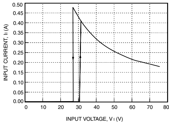
Figure 3. LW010 Input Current vs. Input Voltage at I_{o1} = I_{o, \max} and T_c = 25^\circ\text{C}
