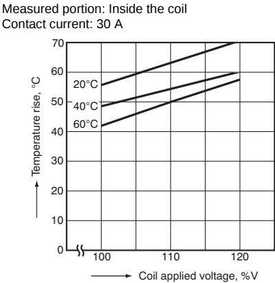
3. Coil temperature rise (DC type)
