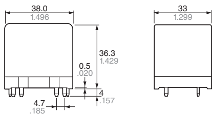
External dimensions
