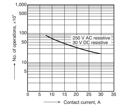
2. Life curve
