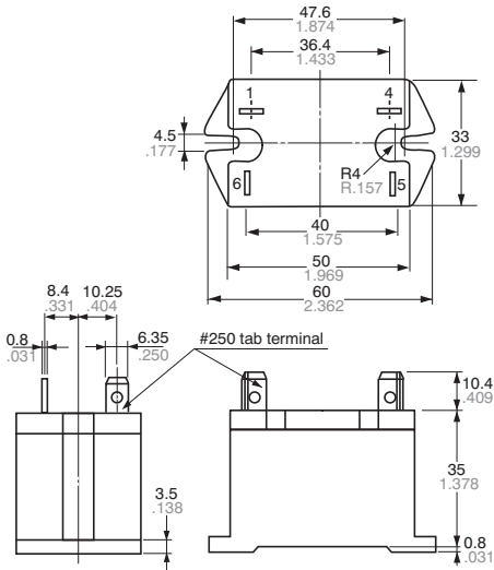
External dimensions Single side stable type 1 Form A
