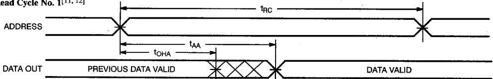
Read Cycle No. 1 [11, 12]
