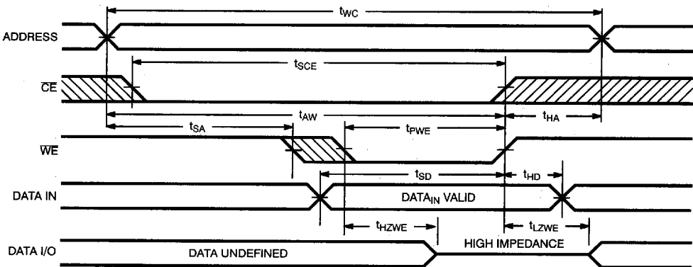
Write Cycle No. 1 ( \overline{WE} Controlled) [10]
