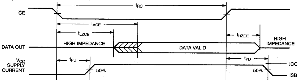
Read Cycle No. 2 [11, 13]
