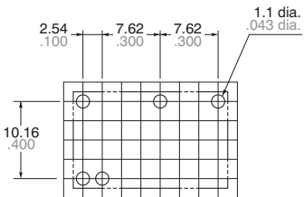
2 coil latching
