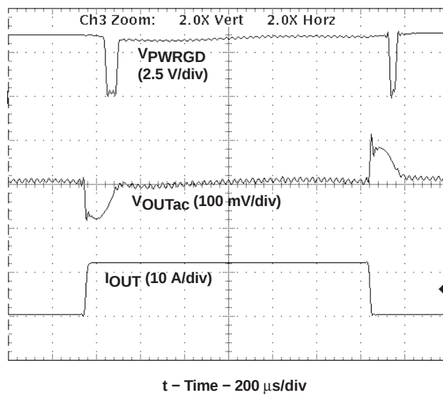
Figure 34. Transient Response
