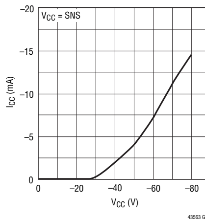
Reverse Current vs Reverse Voltage
