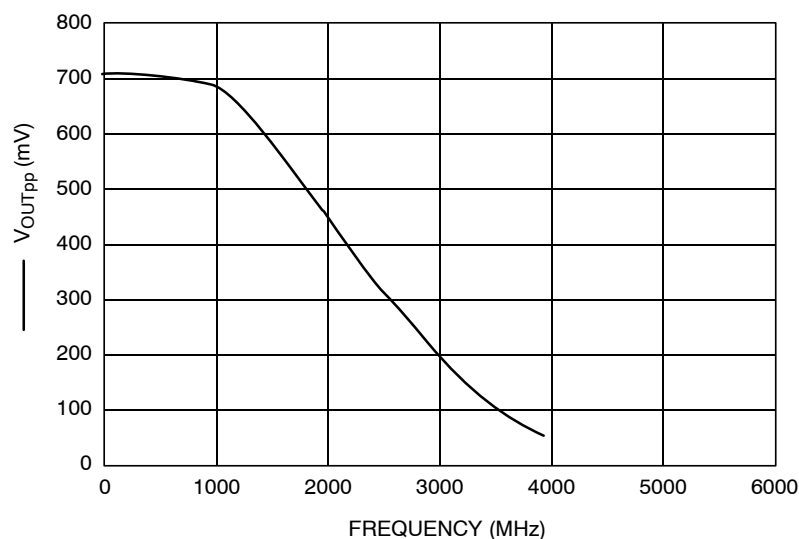
Figure 4. F_{\text{max}} Typical
