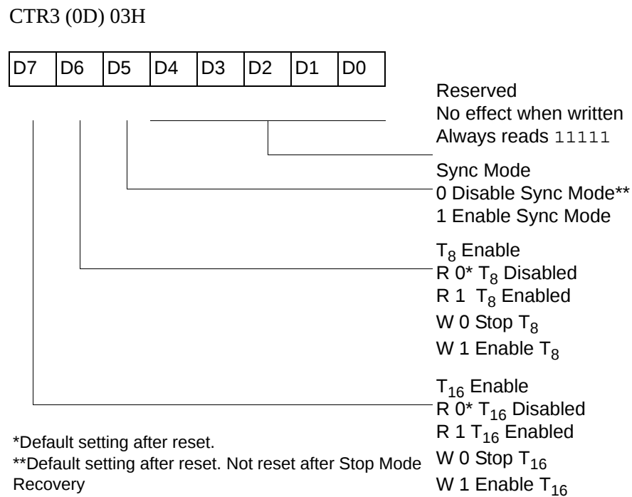
Figure 37. T8/T16 control Register (0D) 03H: Read/Write (Except Where Noted)
