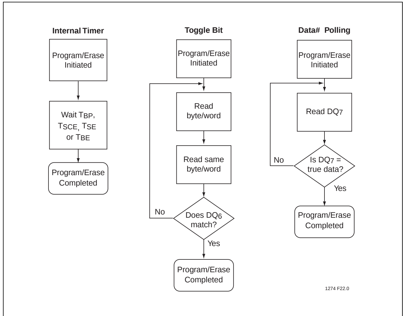
FIGURE 25: Wait Options
