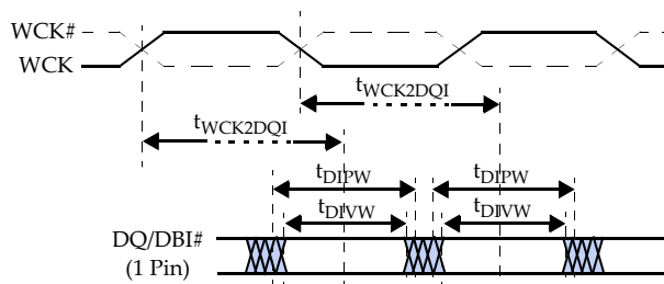
Figure 35. Data Input Timings
