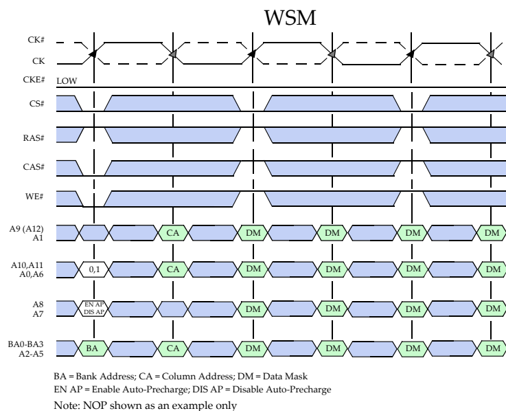
Figure 52. WRITE-With-Singlebyte-Mask Command
