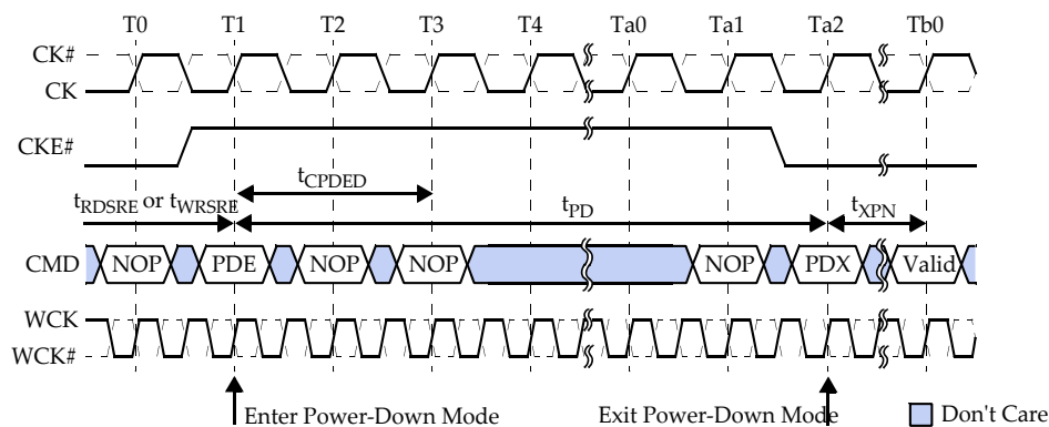
Figure 74. Power-Down Entry and Exit
