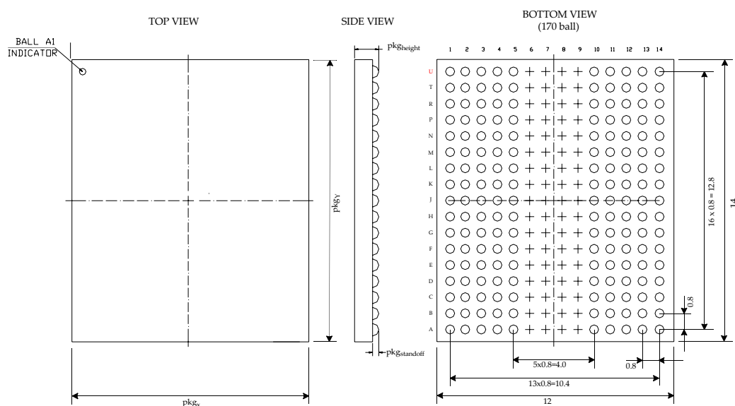
Figure 84. Package Dimensions
