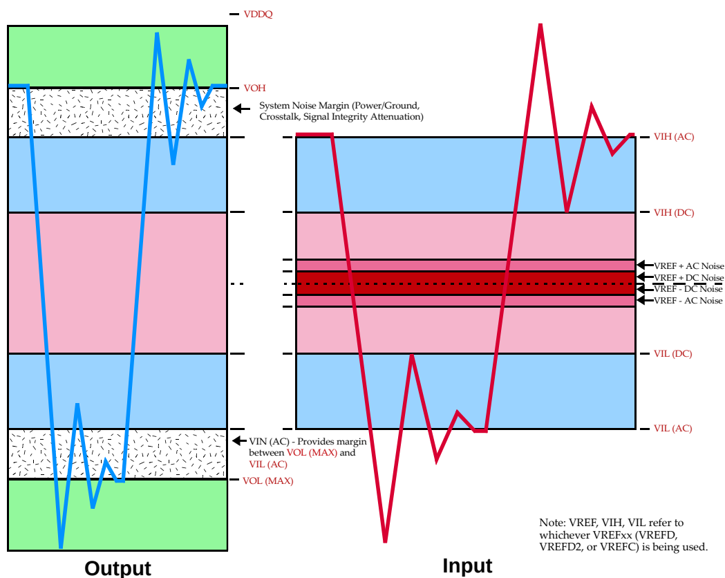
Figure 78. Voltage Waveform
