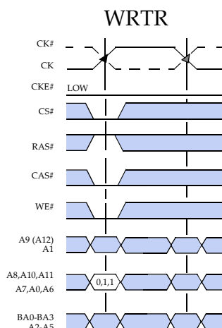
Figure 20: WRTR Command
