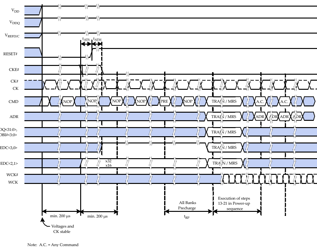
Figure 3: GDDR5 SGRAM Power-up Initialization
