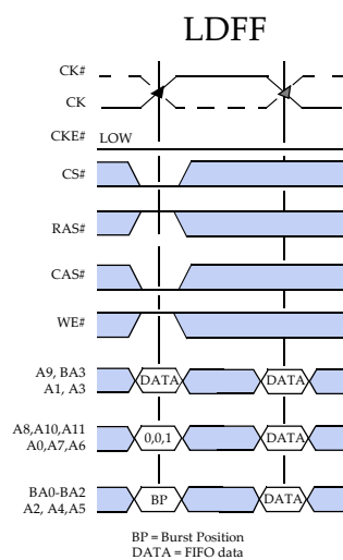
Figure 17: LDFE Command
