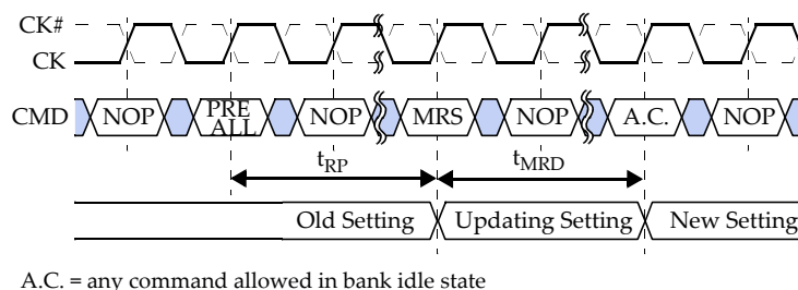
Figure 37. Mode Register Set Timings
