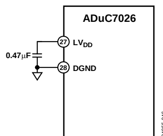
Figure 75. Voltage Regulator Connections
