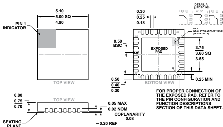
Figure 43. 32-Lead Lead Frame Chip Scale Package [LFCSP] 5 mm x 5 mm Body and 0.75 mm Package Height (CP-32-12)
