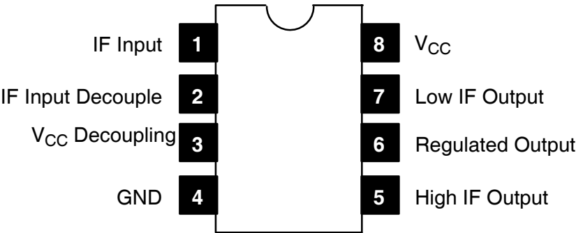
Pin Connection Diagram
