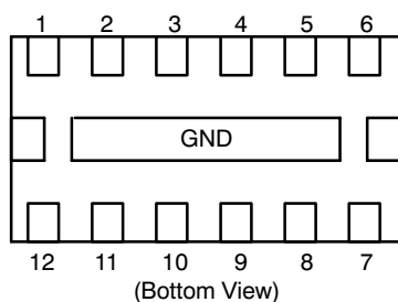
Figure 1. Pin Connections
